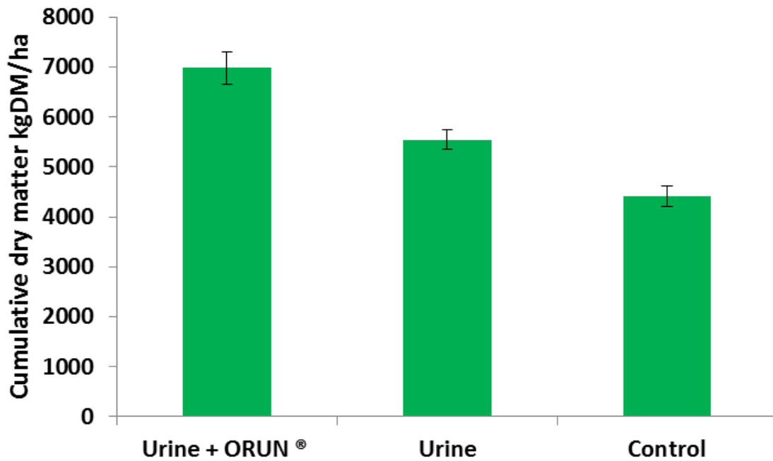
Figure 9. Cumulative dry matter comparison between non urine-treated pasture (control), urine-treated pasture, and urine+ORUN® - treated pasture.
