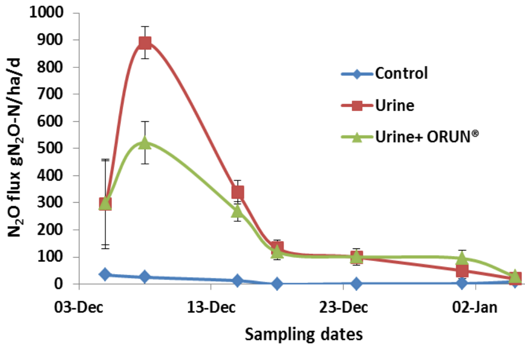
Figure 11. N 2 O flux comparison; control, urine and urine+ORUN®.
