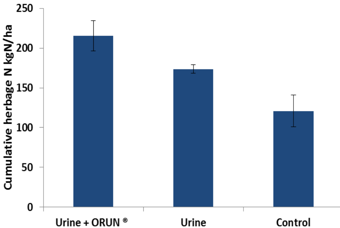
Figure 10. Cumulative herbage N uptake (kg N/ha) comparison between non urine-treated pasture (control), urine treated pasture, and urine+ORUN® treated pasture. Field trial conducted July – Dec 2014.
