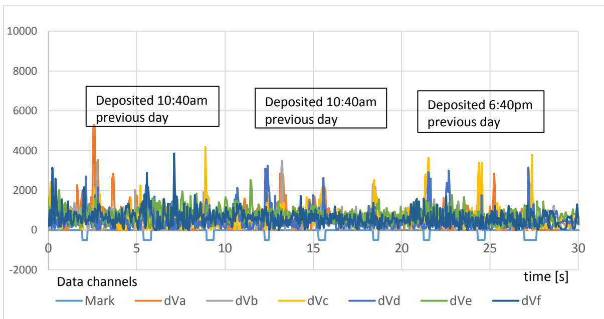
Figure 3. Detection of urine patches placed at various times during the preceding day (same patches as in Figure 2) and detected at 6:20pm, dry soil, damp surface.
