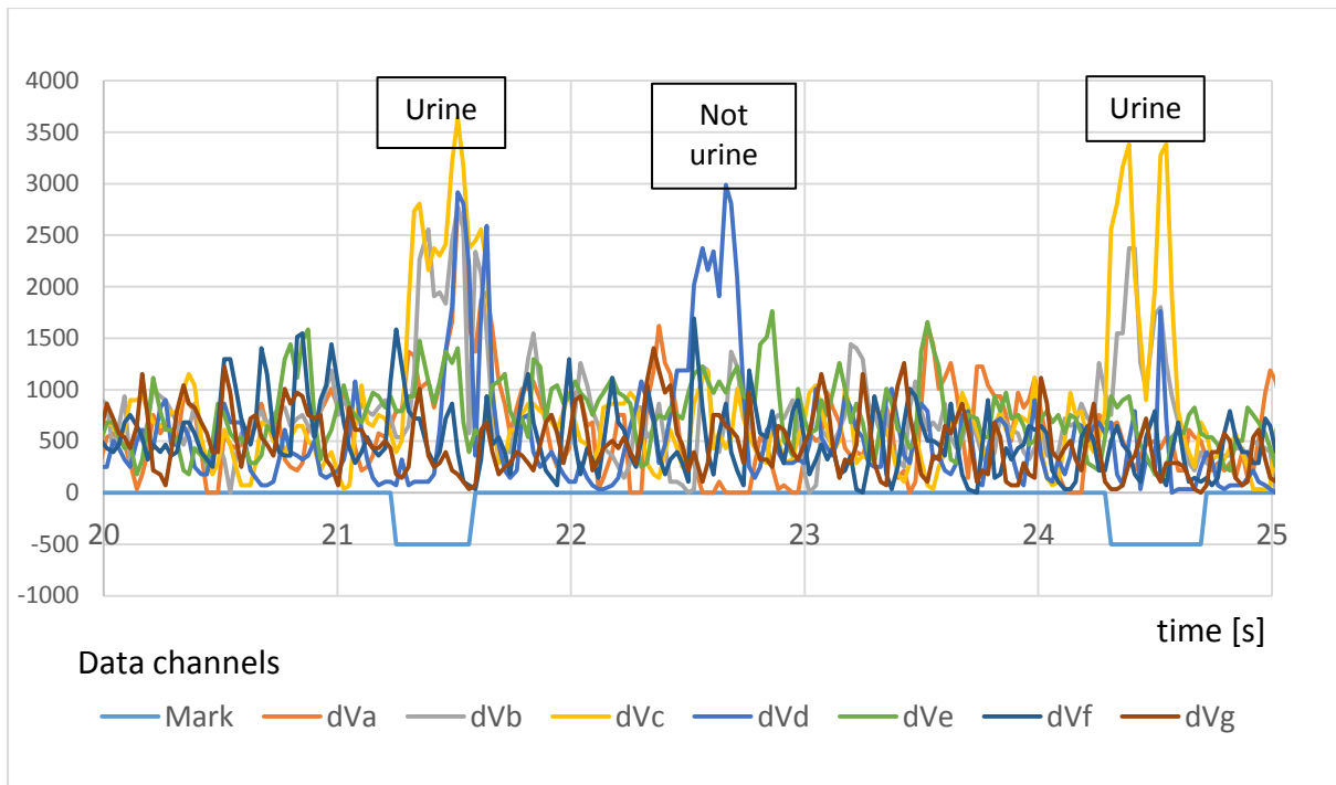
Figure 4. Comparison of response to urine and dung patches, dry soil, damp surface. The signal amplitude is increased with moist soil, as can be seen in Fig. 5, where the data was collected in late spring before this summer’s drought had started.
