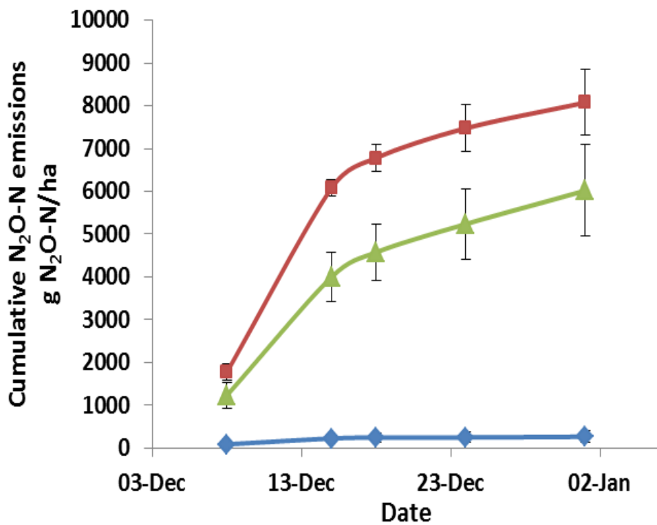
Figure 12. Cumulative N 2 O flux comparison between non urine treated pasture (control), urine treated pasture, and urine + ORUN treated pasture. Field trial conducted Dec 2014-Jan 2015.
