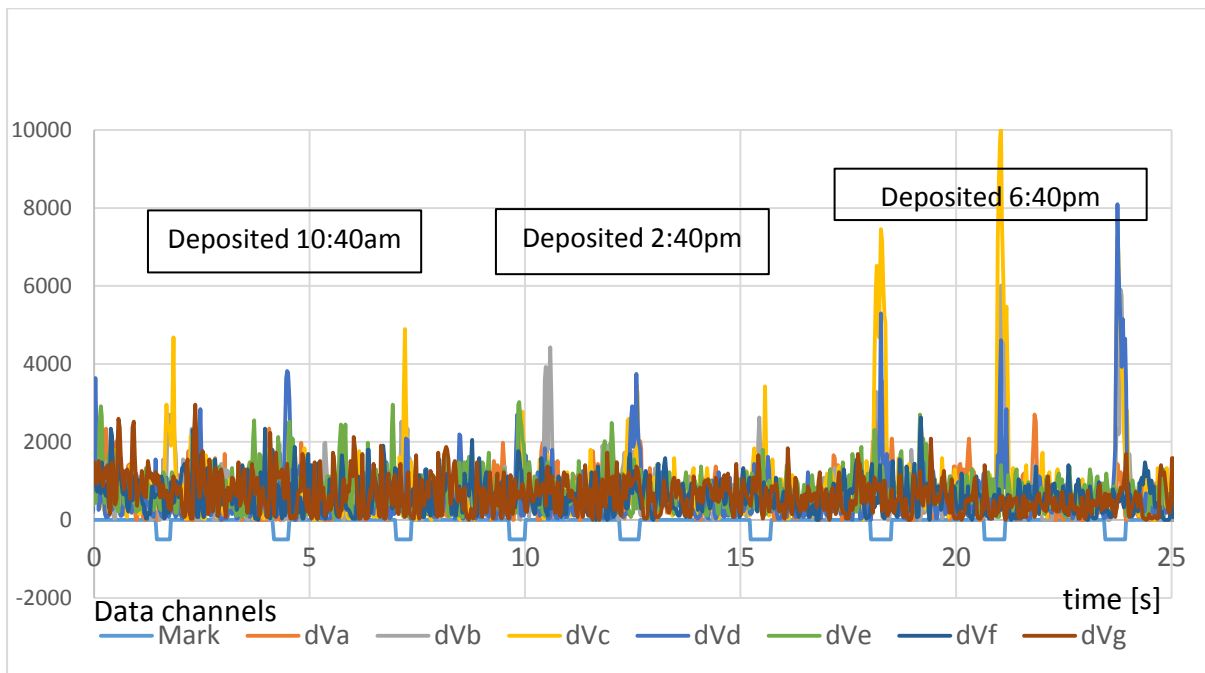
Figure 2. Detection of urine patches placed at various times during the day and detected at 7pm that day, dry soil, damp surface. Blue marks below zero indicate the placement of a urine patch.
