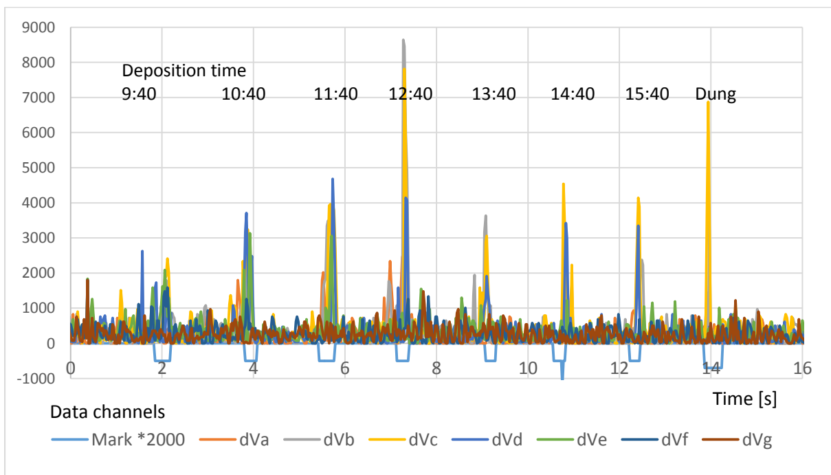
Figure 5. Urine patch detection in moist soil (South Auckland late November) with one dung patch placed at the end of testing. Data taken on the same day as deposition at 5 pm.
